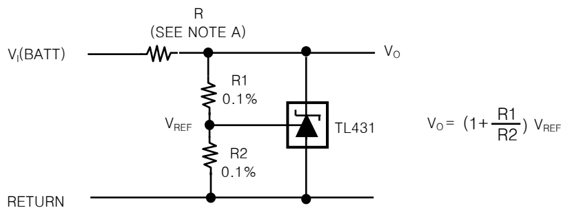
Figure 15. Shunt Regulator
