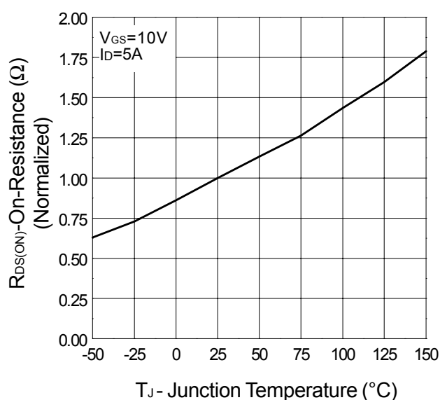
On-Resistance vs. Junction Temperature
