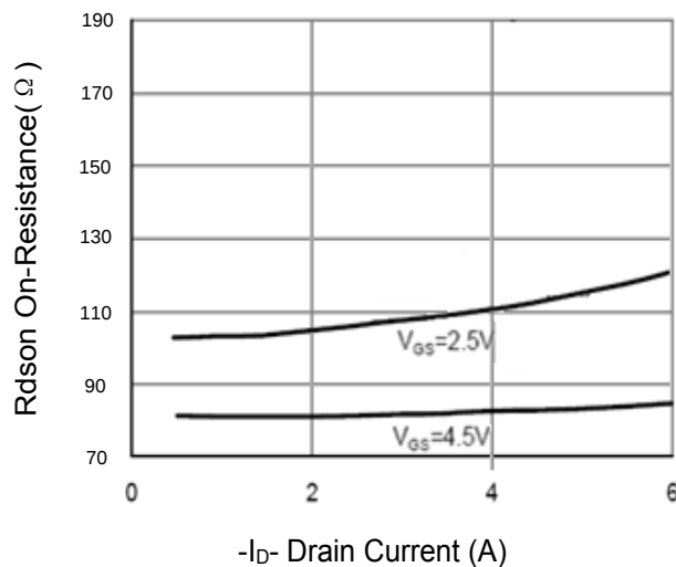
Figure 6 Drain-Source On-Resistance
