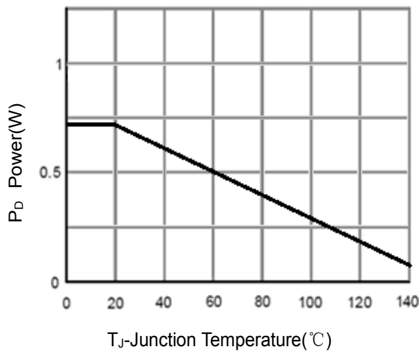
Figure 3 Power Dissipation
