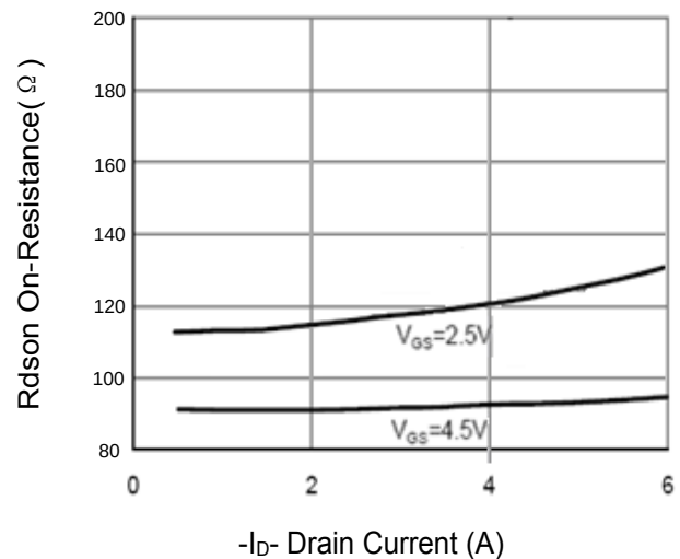
Figure 6 Drain-Source On-Resistance
