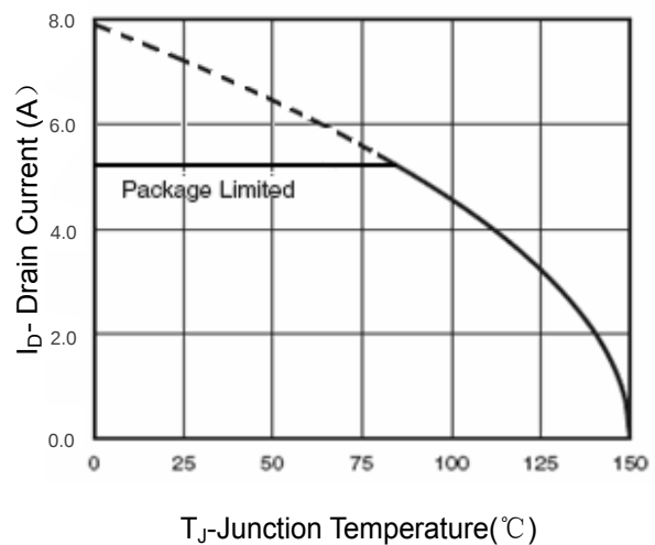
Figure 4 Drain Current
