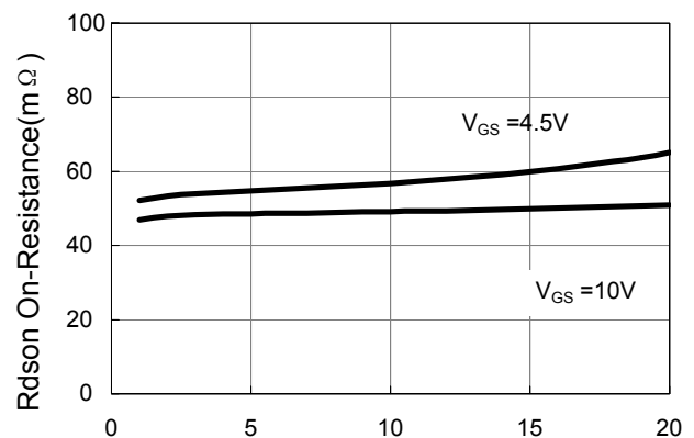
I D - Drain Current (A) Figure 6 Drain-Source On-Resistance
