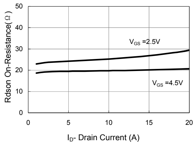
Figure 6 Drain-Source On-Resistance
