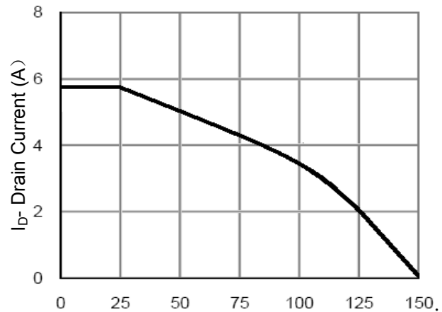
Figure 4 Drain Current
