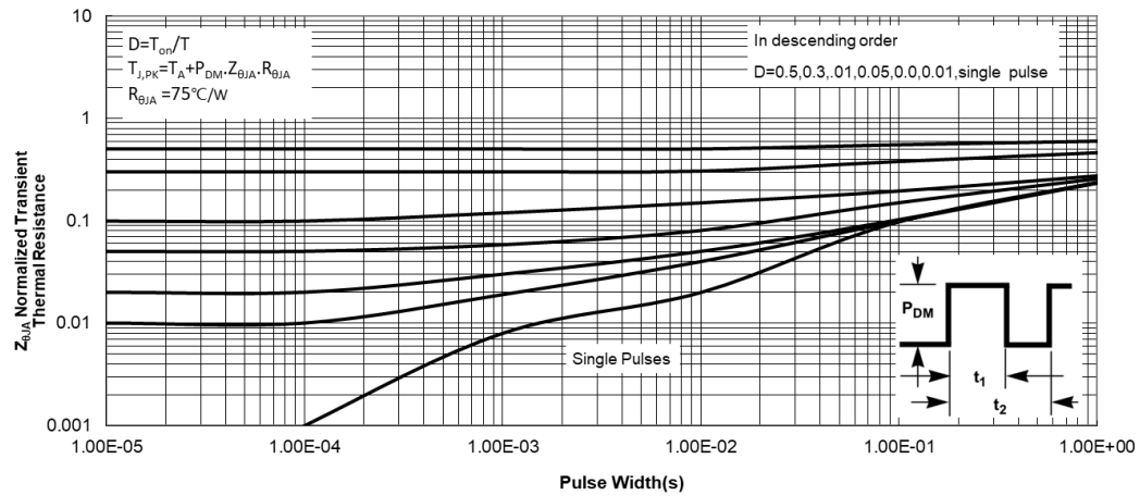
Figure 13. Maximum Effective Transient Thermal Impedance
