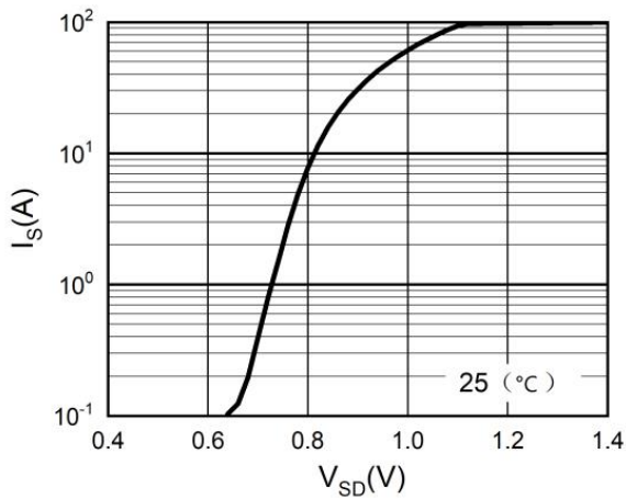
Figure 9. Body-Diode Characteristics
