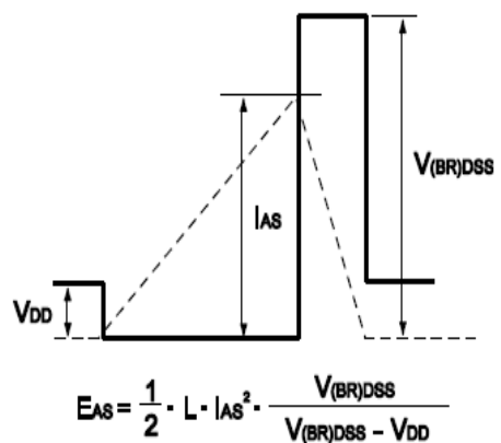
Avalanche Waveform
