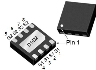
DFN3030-8L
