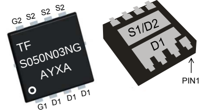
DFN5x6-8L
